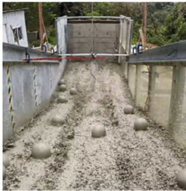
Testing of Debris Impact (泥石流撞擊試驗)
